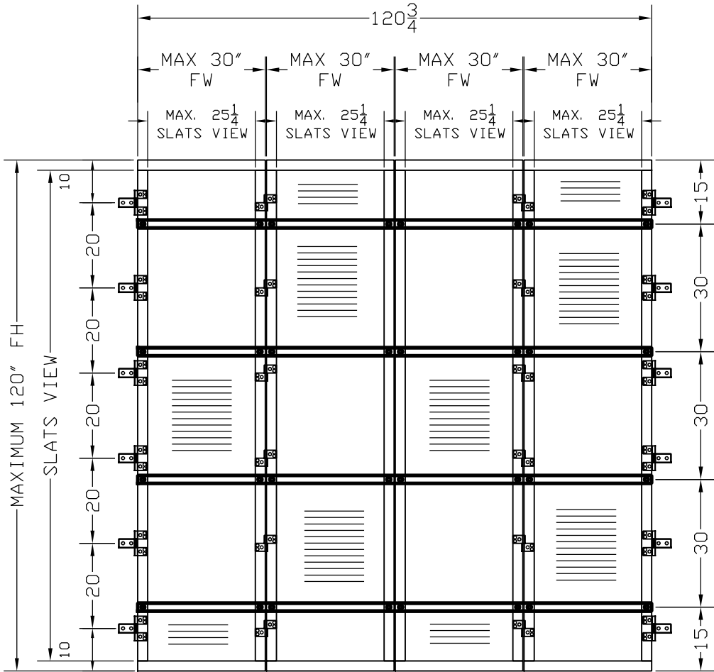
TYPICAL 4 PANELS ELEVATION
